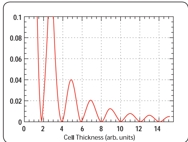
Fig. 4-3 Liquid crystal cell thickness changes
