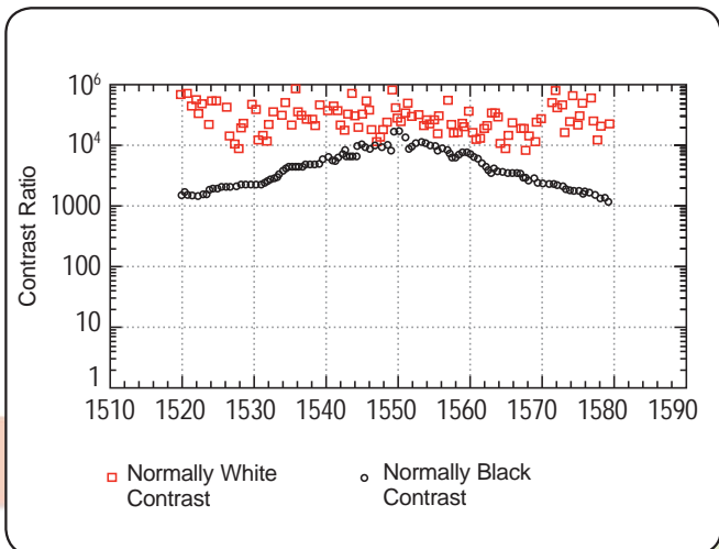
Fig. 4-4 Contrast ratio for a twisted nematic liquid crystal cell
