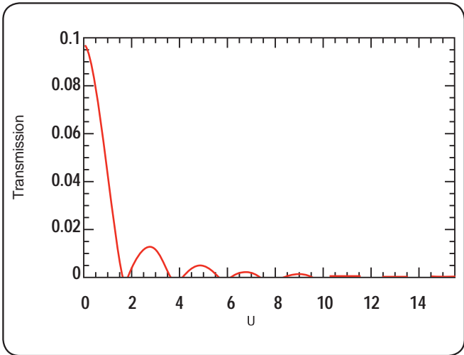
Fig. 4-2 Transmission of a twisted-nematic cell between parallel polarizers as a function of thickness and/or wavelength
