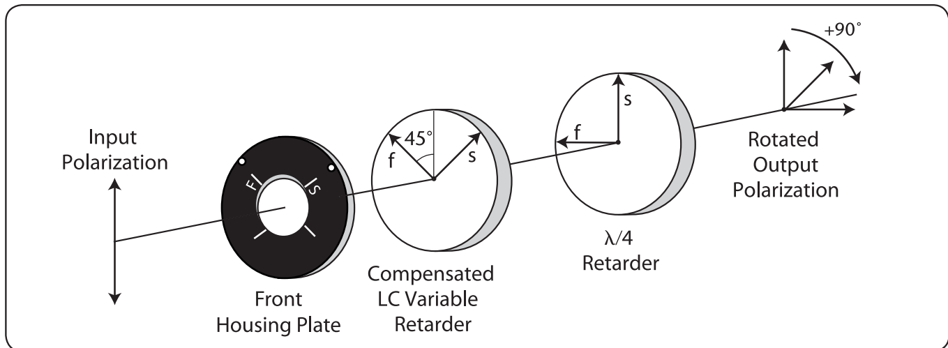
Fig. 4-15 Operation of Liquid Crystal Polarization Rotator showing complete rotation of a linearly polarized input beam
