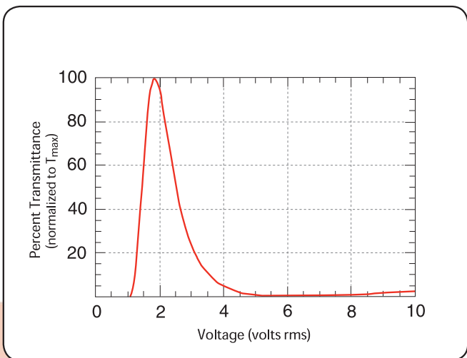
Fig. 4-12 Normalized transmittance of Liquid Crystal Variable Attenuator with crossed linear polarizers at a single wavelength
