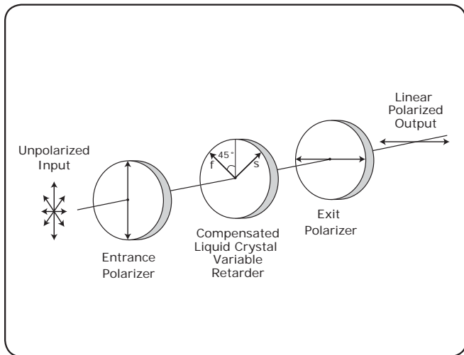
Fig. 4-11 Standard Liquid Crystal Variable Attenuator design uses crossed linear polarizers
