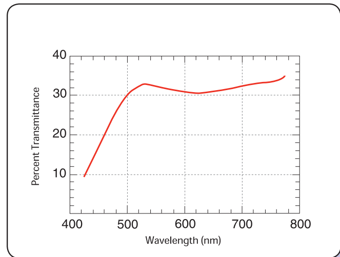
Fig. 4-13 Unpolarized Transmittance as a function of wavelength for LC Variable Attenuator, optimized for 550 nm, with polarizers and unpolarized input
